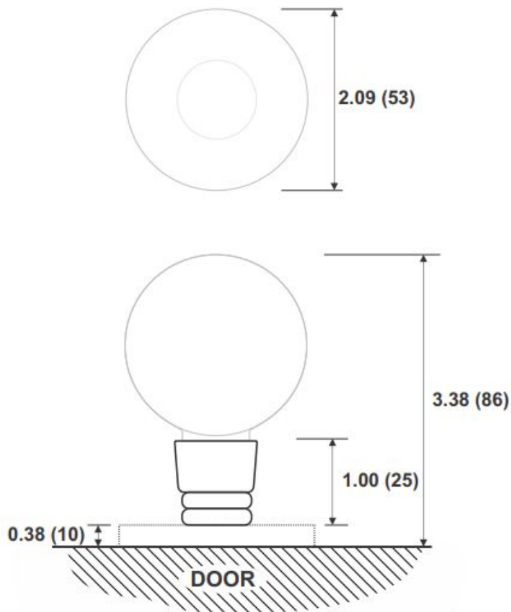
BRISTOL KNOB (BL)
