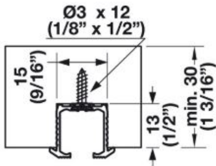
Top track, screw mounting
