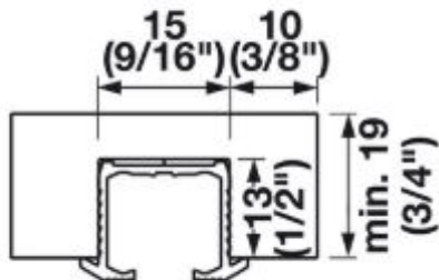
Top track, for gluing into groove
