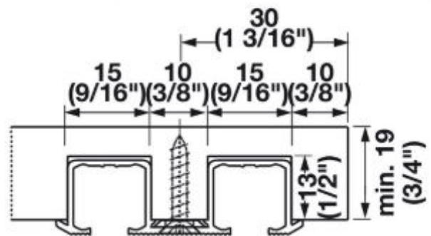
Dual top track, screw mounting
