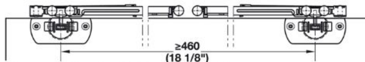
Door with two Soft Close mechanisms.
