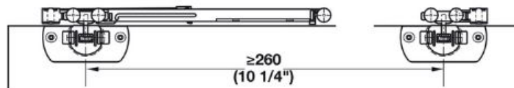
Door with one Soft Close mechanism.
