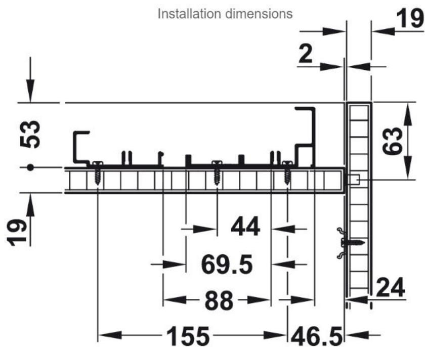
Section running track without running gear, top
