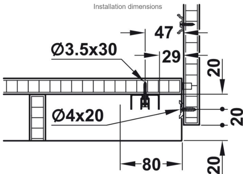
Section running track without running gear, bottom
