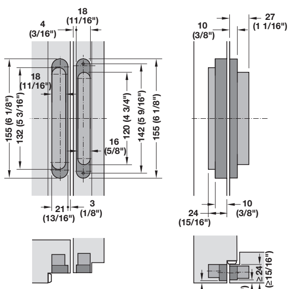
Milling template for a wood door frame
