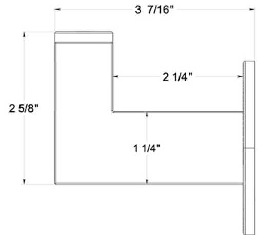
PROFILE VIEW
